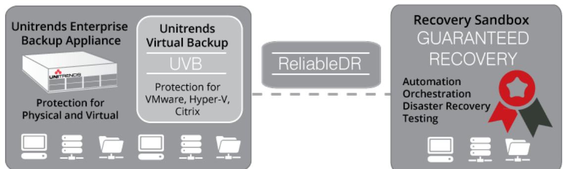
UCRS Architecture
