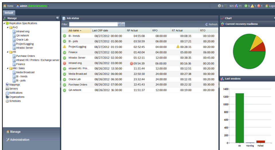
ReliableDR Interface
